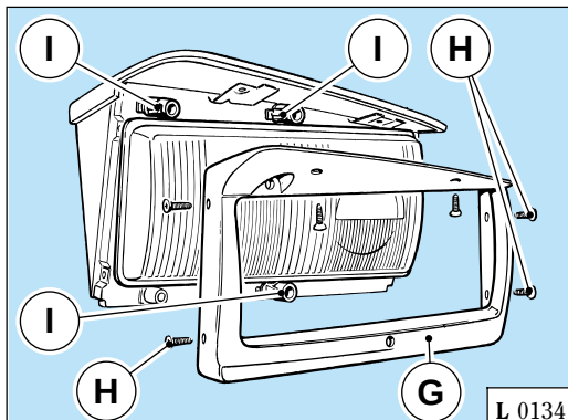
Fig. 7 - Replacement of bulbs.
