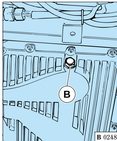
Fig. 6 - Oil change
