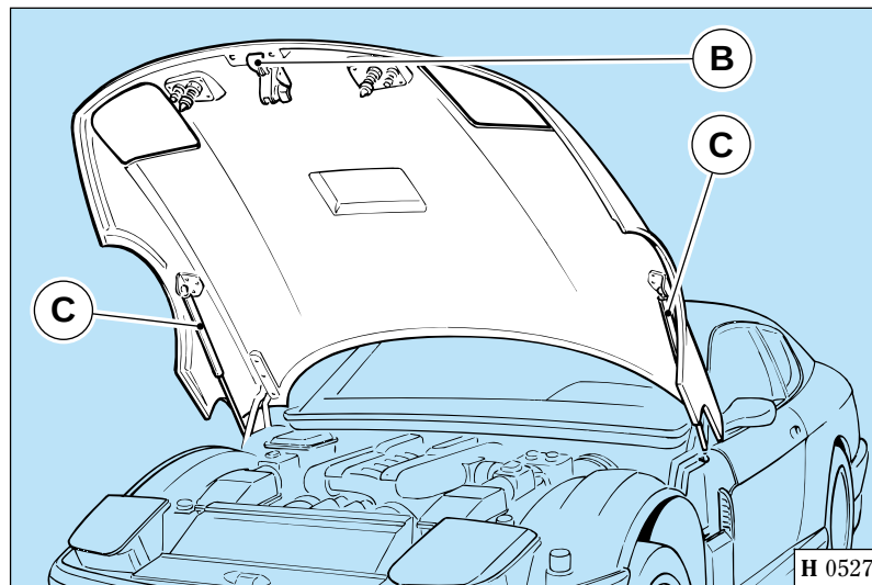
Fig. 32 - Engine hood
